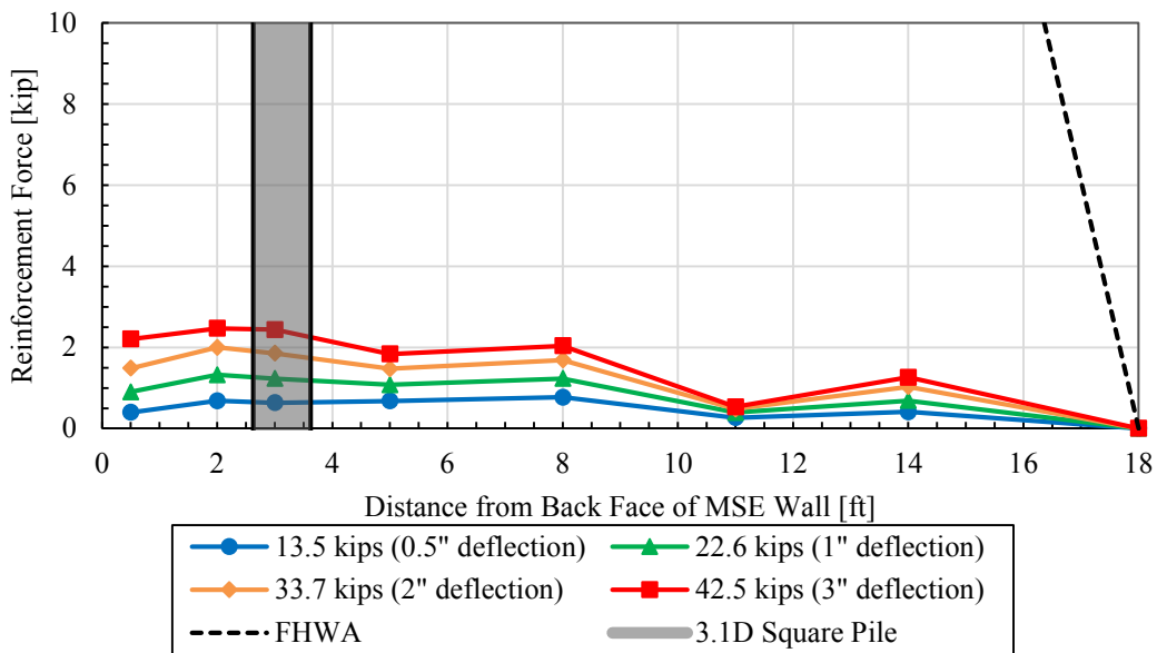
Figure D-28. Reinforcement force versus distance from back face of MSE wall (square pile 3.1D, 15-inch depth, welded wire #2, transverse spacing 44 inches).
