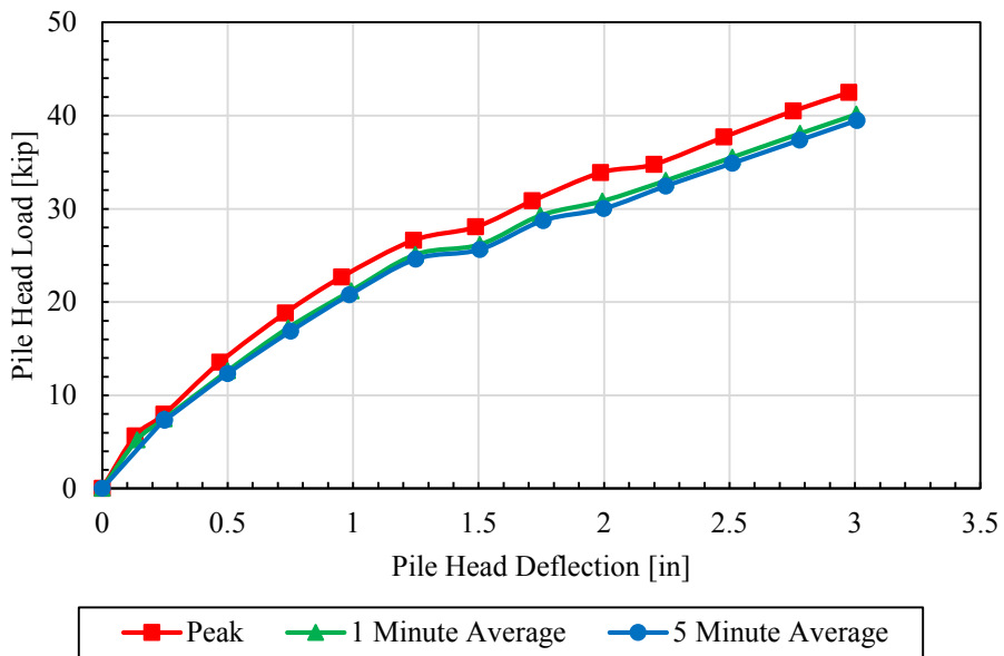
Figure C-8. Pile head load versus pile head deflection comparing peak, 1-minute hold, and 5-minute hold for 2.1D square pile.
